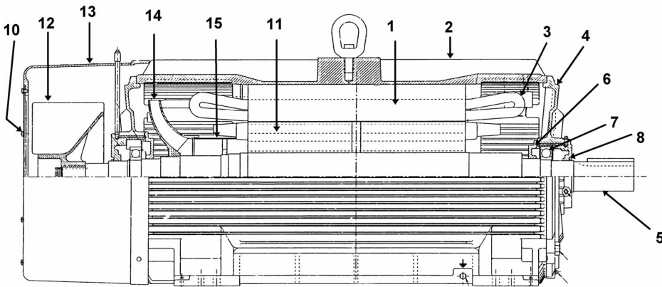
Figure 14. Type CZ, 588 / 5810 / 5812 Frames
