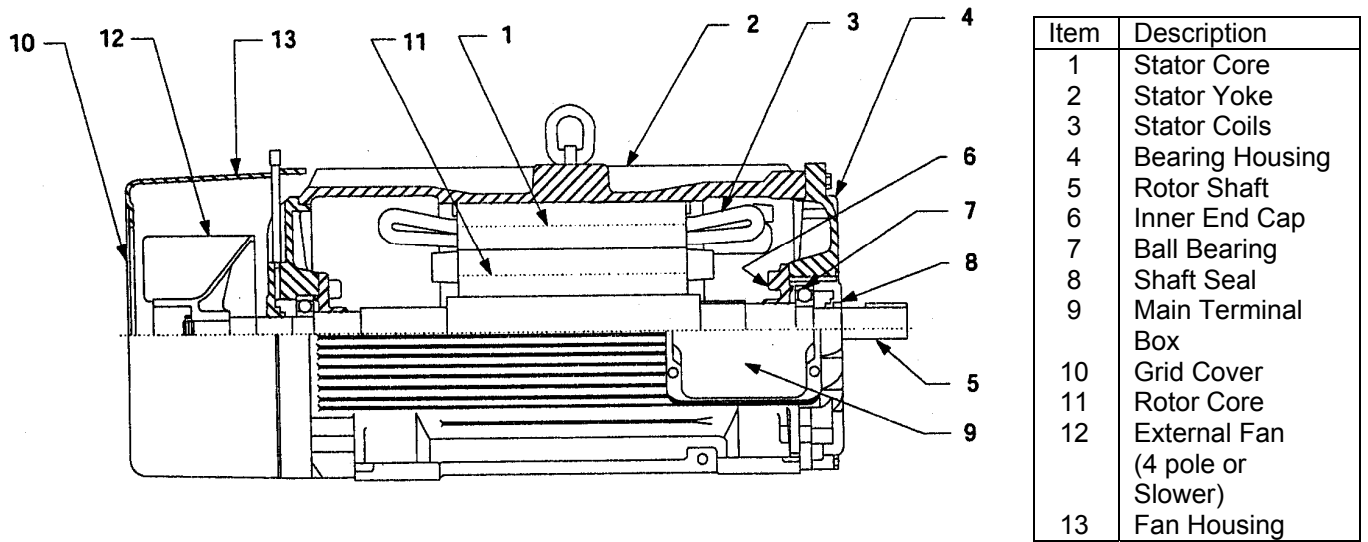
Figure 11. Type CGZZ, 507, 509, and 5011 Frames. (U.L. LISTED)
